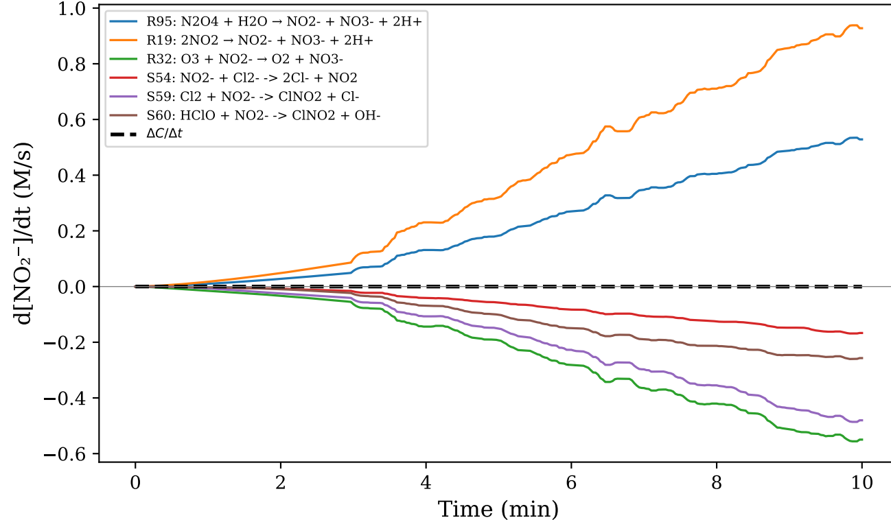
(c) \text{NO}_2^-
